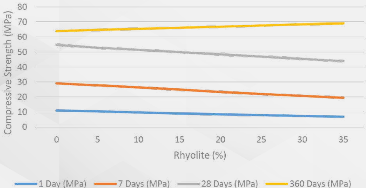
Effect of Rhyolite on Compressive Strength
