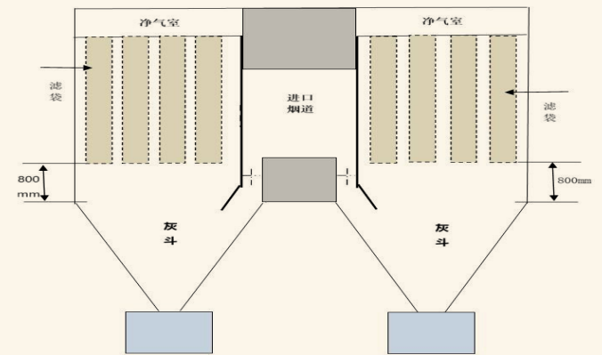
Figure 5 Front Sectional View of the Dust Collector Inlet
